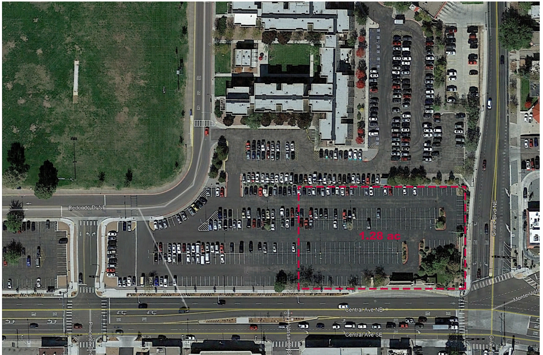
Proposed Site Development for Central Ave. & Girard Blvd. Target Store Location 6/25/19
